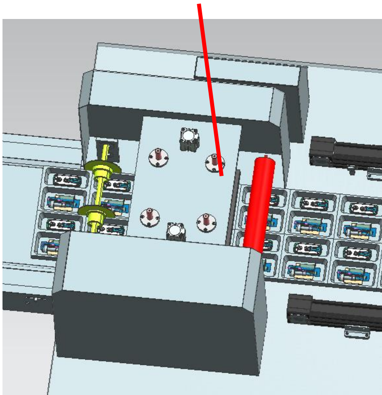
Horizontal & tear notch cutting
